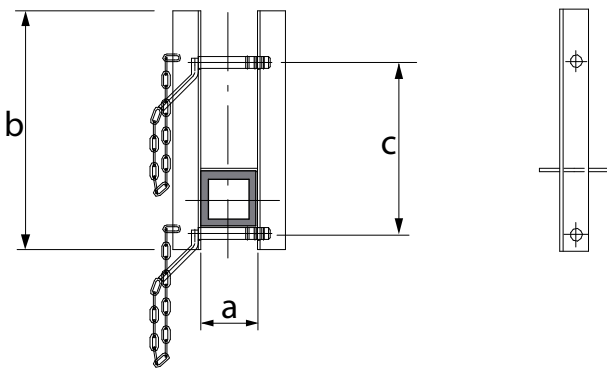
Mounting rig H10
